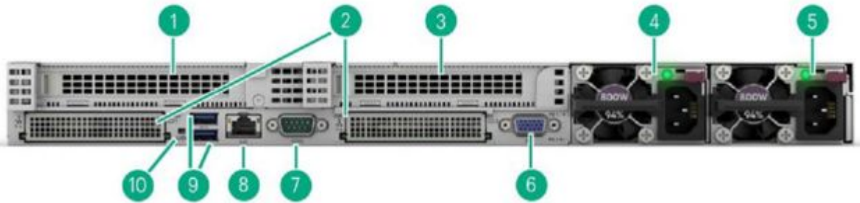
Rear View - Standard for all DL365 Gen11
